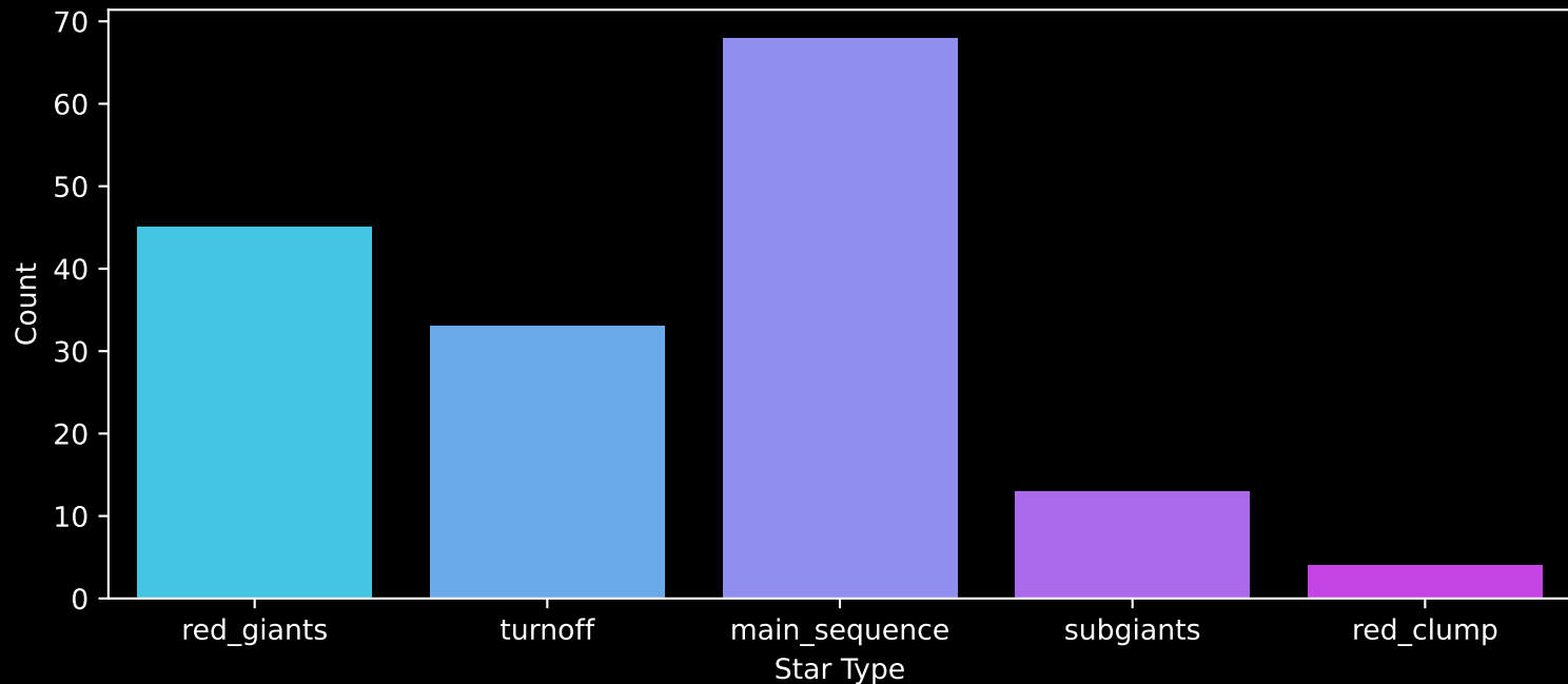
APOGEE DR17 Field: [273-35-O_TESS] Count plot of Star Type
