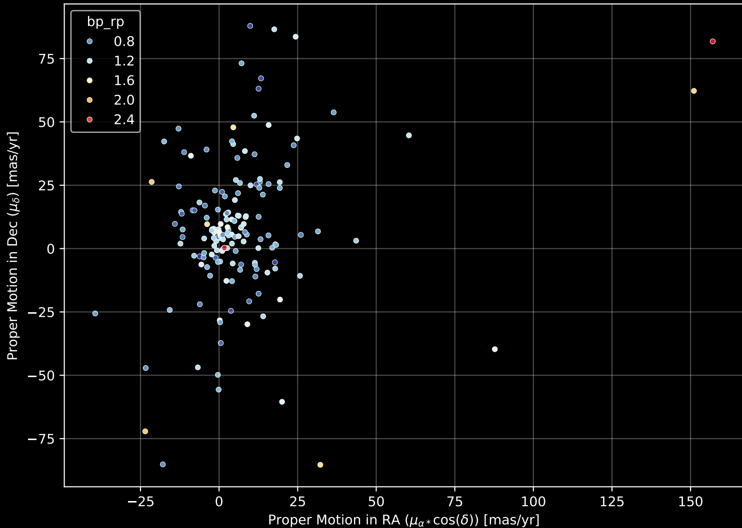
APOGEE DR17 Field: [273-35-O_TESS] Proper Motion Diagram (n= 163)
