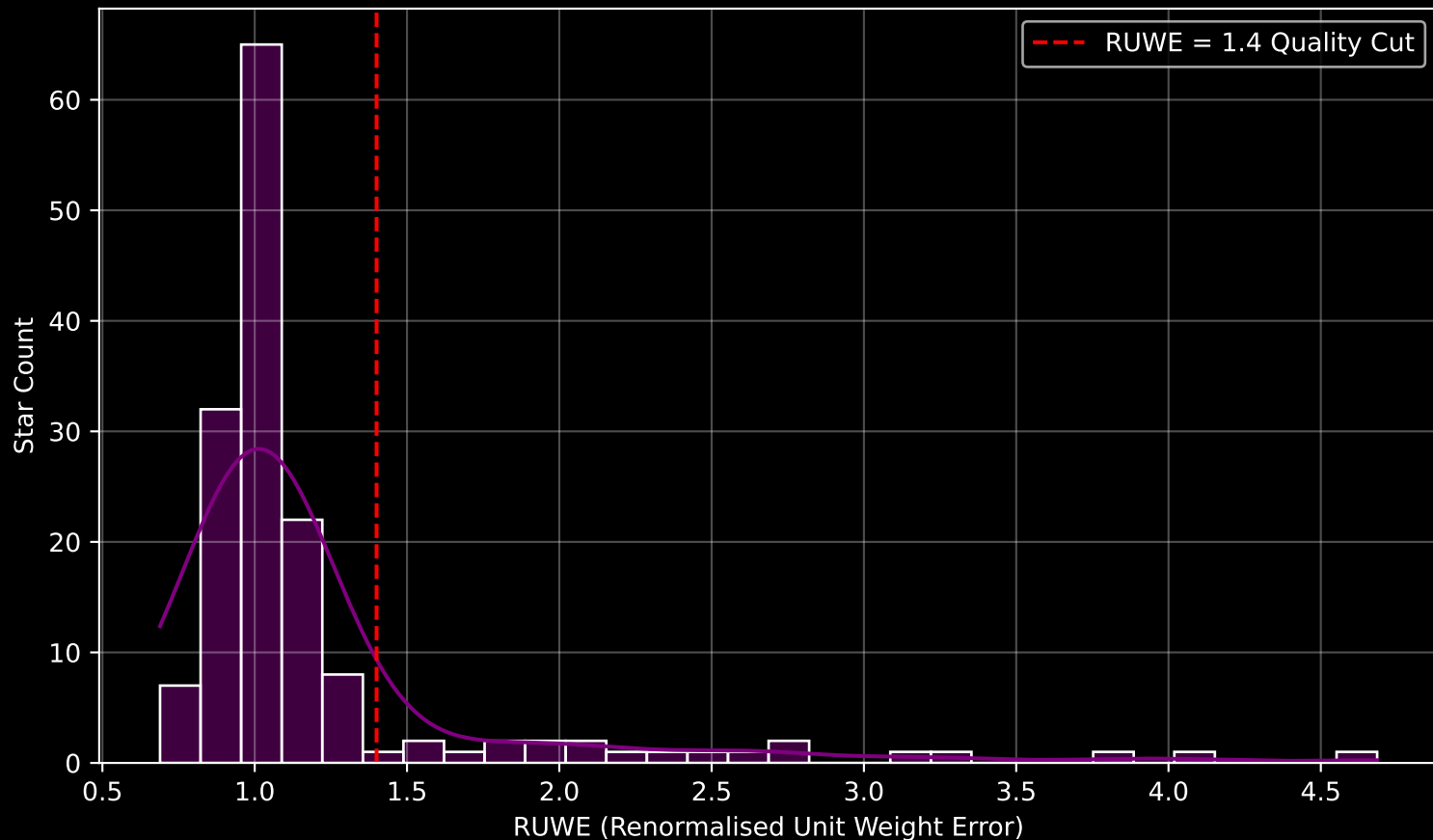
GAPOGEE DR17 Field [273-35-O_TESS] RUWE Distribution (n= 155)
