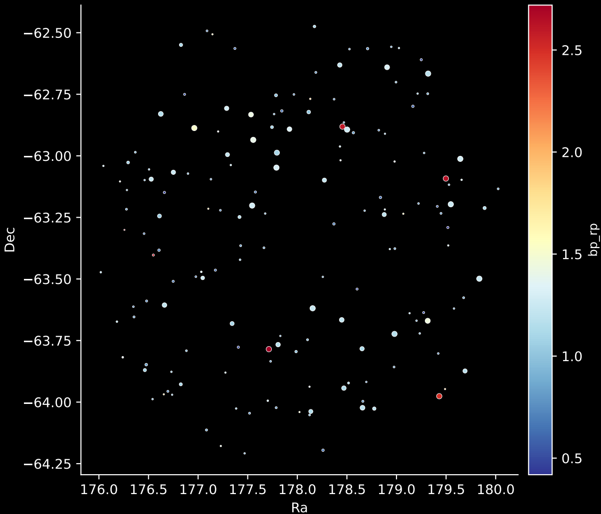
APOGEE DR17 Field: [273-35-O_TESS] Stars: 163
