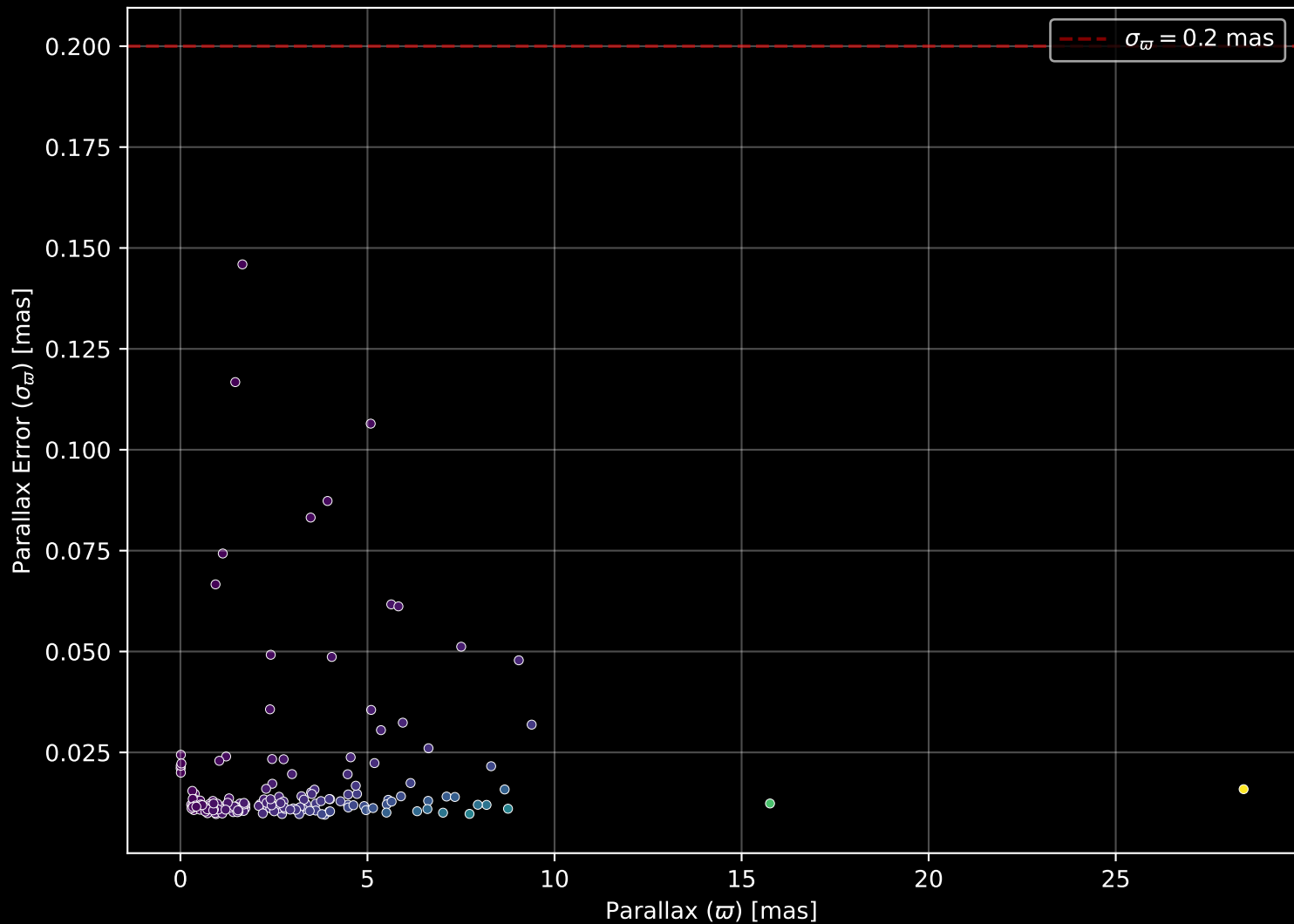
APOGEE DR17 Field: [273-35-O_TESS] Parallax Quality (n= 163)
