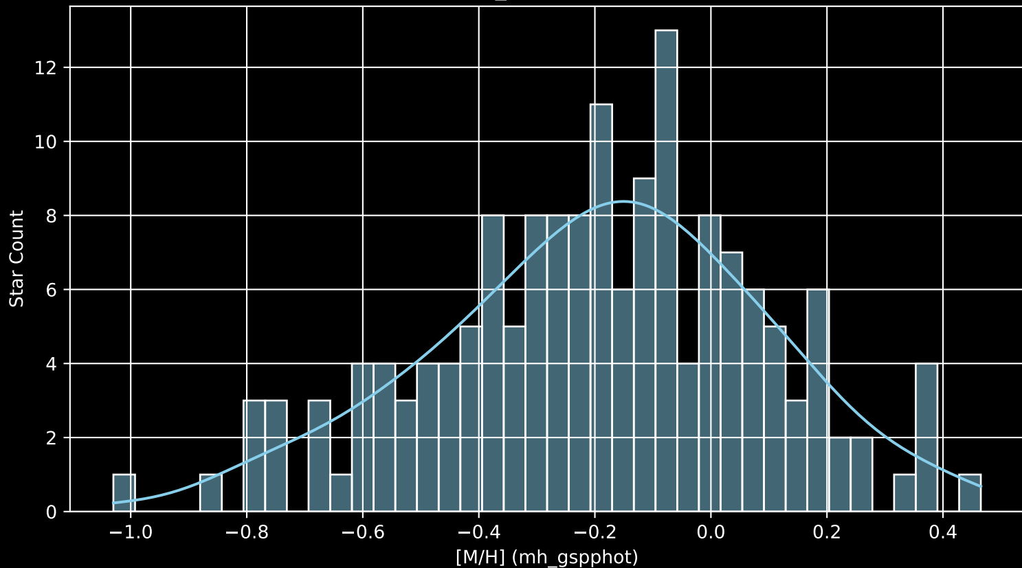
APOGEE DR17 Field: [273-35-O_TESS [M/H] (mh_gspphot) (n= 161)
